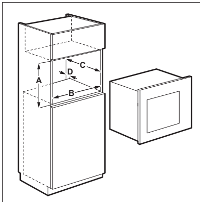
Installation distances
